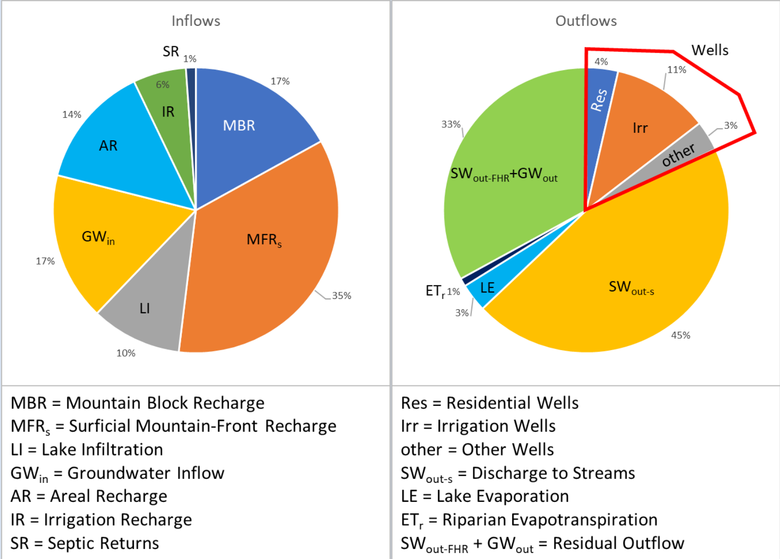
Relative Groundwater Budget (Berglund and others, 2024) Total Annual In/Out ~60,000 ac-ft/yr
